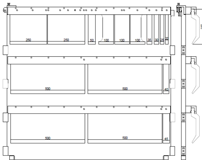
Optional rails configuration, 3 cassettes
