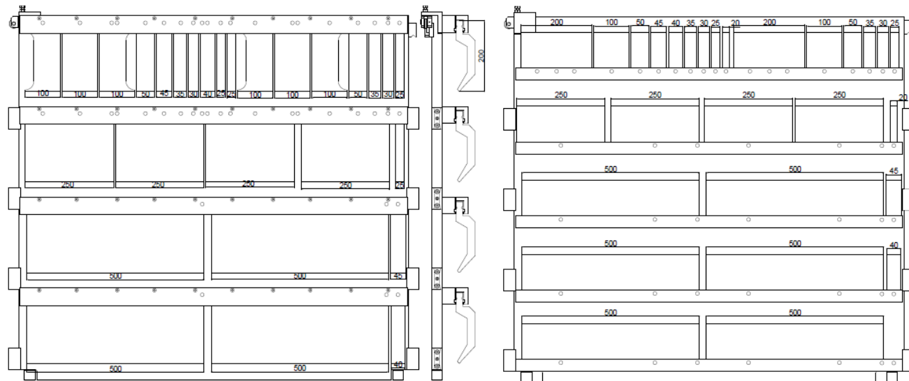
Standard upper tool rails, 4 cassettes
